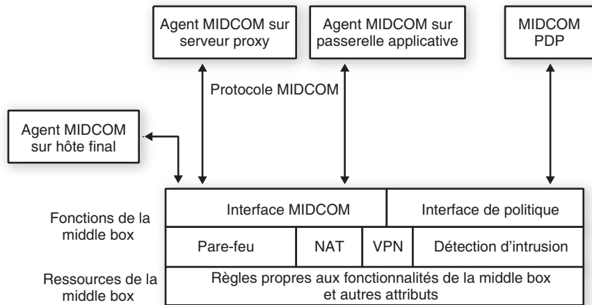
Figure Q.35 Architecture d'une middle box
